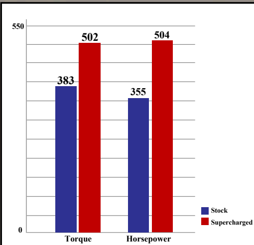
SUPERCHARGED FLYWHEEL HORSEPOWER and TORQUE (ft-lbs) 2015 5.3L GM SUV
