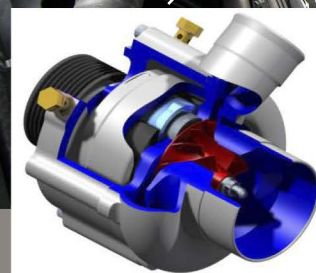
Supercharger cut-away
