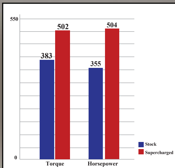
SUPERCHARGED FLYWHEEL HORSEPOWER and TORQUE (ft-lbs) 2016 5.3L GM Truck
