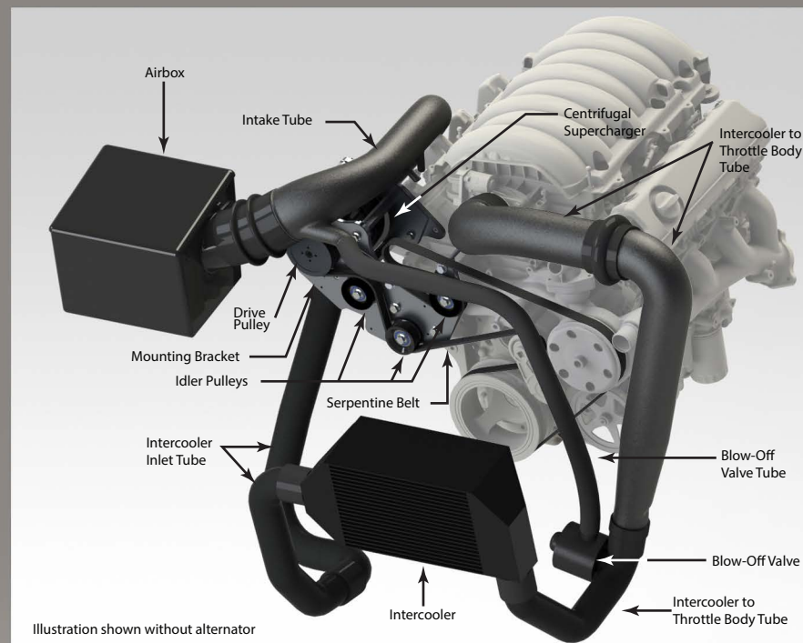
Supercharger main components
