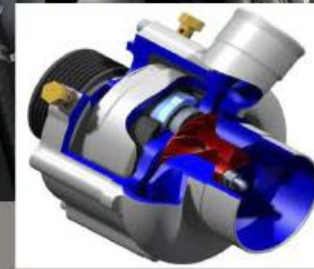
Supercharger cut-away
