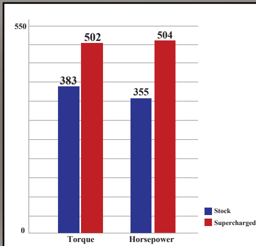
SUPERCHARGED FLYWHEEL HORSEPOWER and TORQUE (ft-lbs) 2016 5.3L GM SUV
