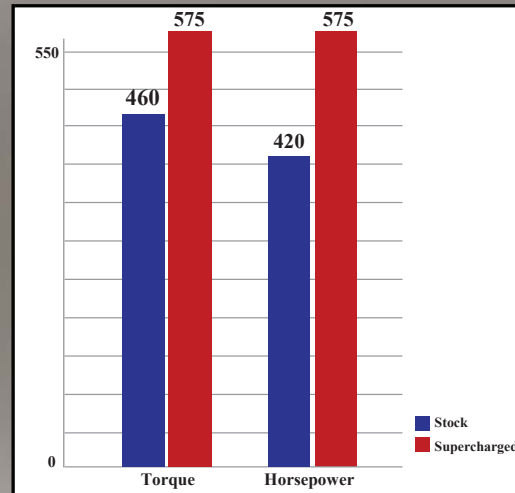
SUPERCHARGED FLYWHEEL HORSEPOWER and TORQUE (ft-lbs) 2016 6.2L GM SUV
